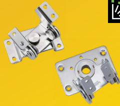
Dual Axis Torque Hinges HG-T30S15, HG-T70S30
